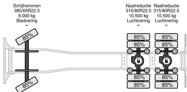
Mercedes-Benz Arocs 2658 2858 | 6X4 EURO 6 BIG AXLES |...
