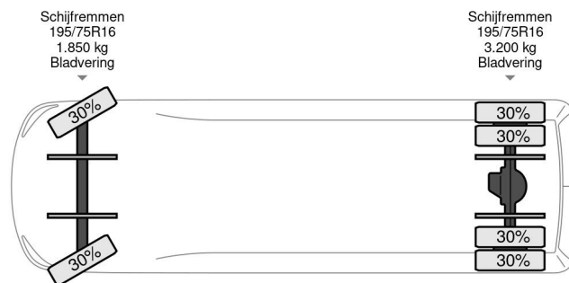
Renault Master 160 DCI | L3H3 | WORKSHOP | WERK... 4x2
