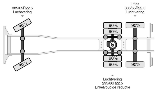
Scania R490 | 6X2 | RETARDER | BDF | MOBILE WORKSH...
