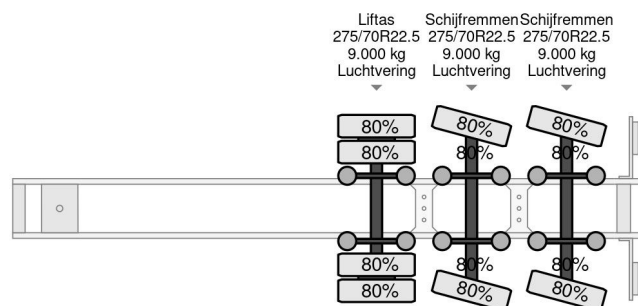
Kelberg HIAB 228-4 | 3 AXLE | LIFT AXLE | 2X STEERING | ...
