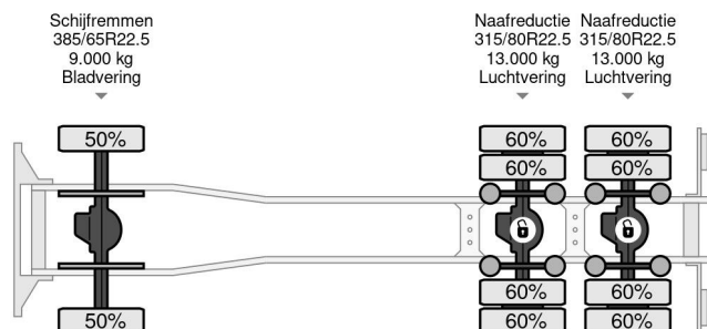
MAN TGS 26.500 | 6X6 | HYDRODRIVE | BIG AXLES | EURO 6
