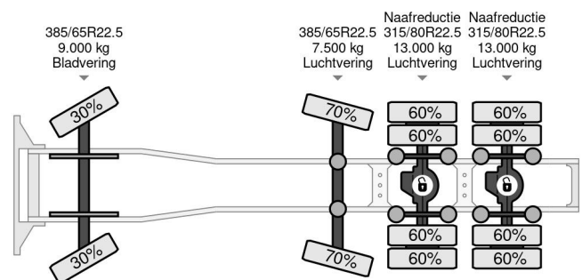
MAN TGX 41.640 | 8X4 | 150 TON! | RETARDER | HYDR | B...
