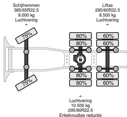
Scania R500 NGS | 6X2 | RETARDER | FULL AIR | EURO 6
