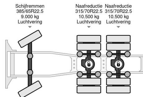
Scania R580 V8 | 6X4 | HYDRAULICS | RETARDER | 85 TON...
