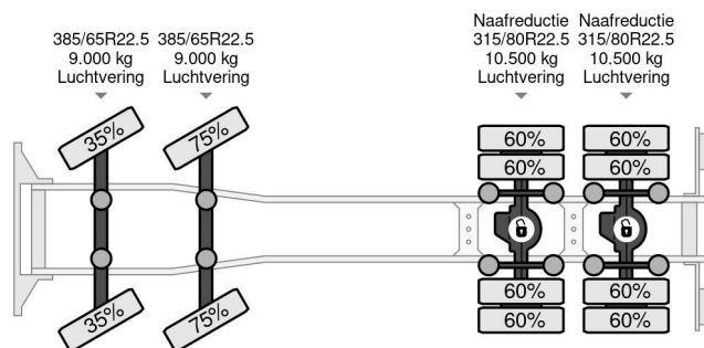
Scania R580 V8 8X4 RETARDER BIG AXLES HOOKLIFT F...
