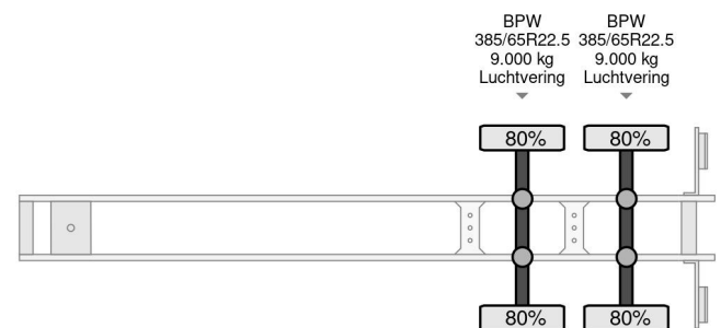
Zaslaw 2 AXLE OPEN TRAILER + FASSI F185-4 (YEAR 202...
