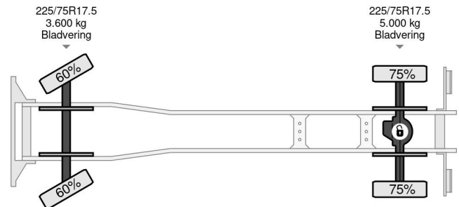
DAF LF 210 | 4X2 | PALFINGER PK5001 | REMOTE | 48.000...
