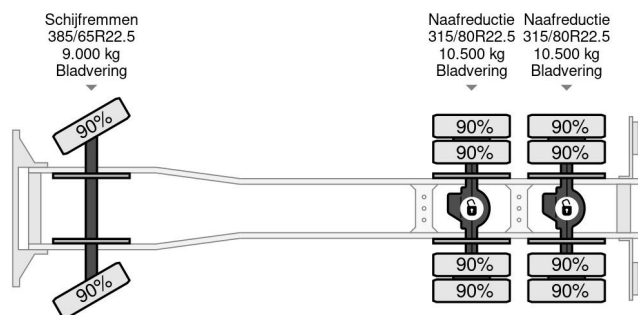
Scania R580 V8 | 6X4 | FULL STEEL | BIG AXLES | RETARD...
