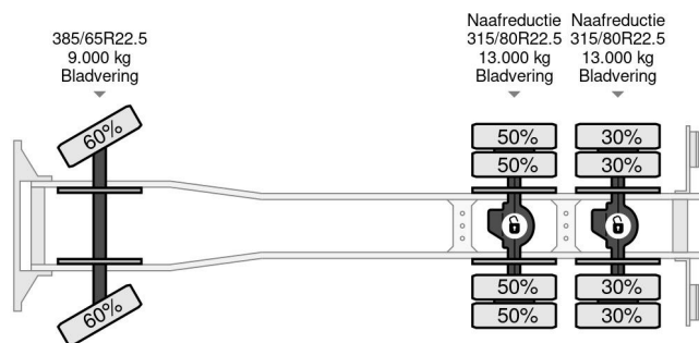
MAN TGA 33.480 6X4 | HIAB 166E-5 | KIPPER | FULL STEEL
