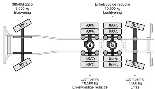
Volvo FM 500 8X4 TRIDEM + HIAB 477 E-6 HIPRO | REMO...
