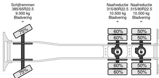
Iveco Stralis X-WAY 570 6X4 FULL STEEL BIG AXLES RET...
