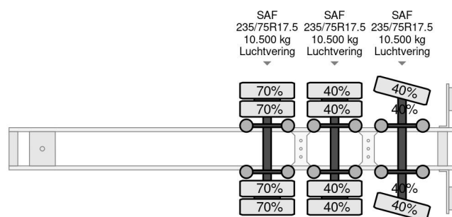
Max Trailer MAX 100 | 3-AXLE | LIFT DECK | SLIDING RAMPS
