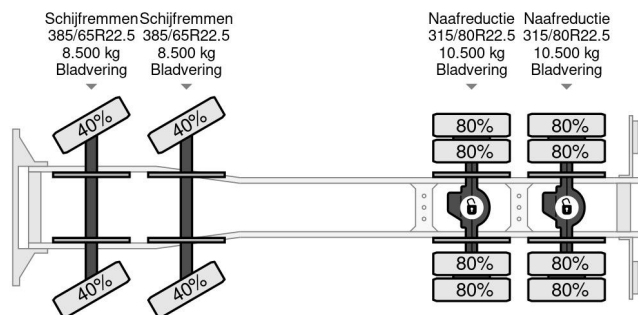
Scania R580 V8 | FULL STEEL | BIG AXLES | RETARD... 8x4
