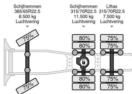
Volvo FH 13.540 | 6X2 | RETARDER | ADR | EURO 6
